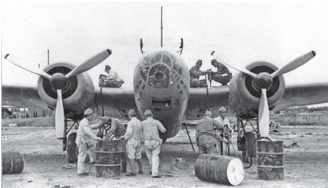
A Ki-21-II being refuelled from hand-pumps mounted on tripods, a laborious process which could take several hours. Ki-21s were among the replacement aircraft that arrived in Wewak from the Philippines in September 1943.
